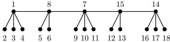
Figure 2: A caterpillar and its corresponding permutation.
