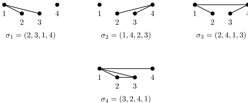
Figure 1: Permutation graphs.
